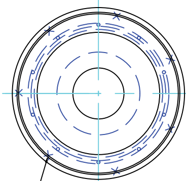
VENTURI & COLLAR WELDED 5 PLACES, 72 DEGREES APART.
