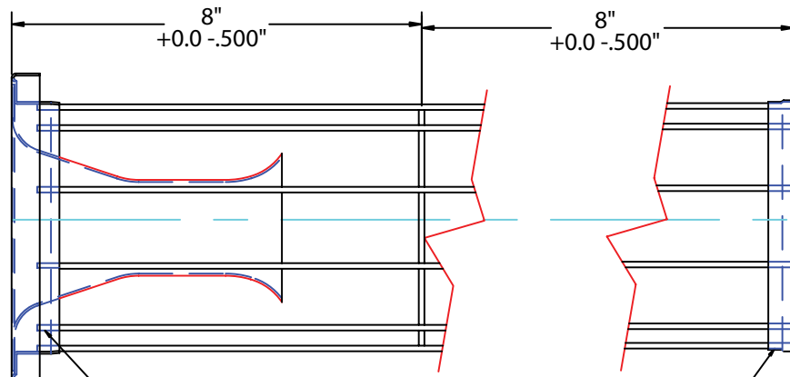
COLLAR WELDED 10 PLACES TO VERT. CAGE WIRES
